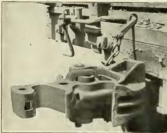
EMERGENCY KNUCKLE IN USE.
